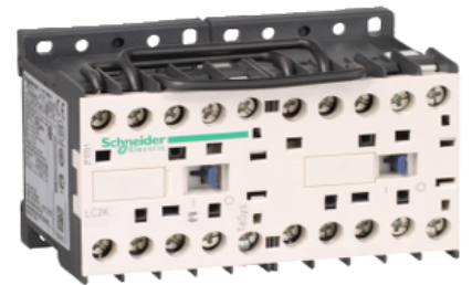
SCHNEIDER ELECTRIC 4KW 9A 1NC INVERTER CONTA- CTOR 48VAC CONTROLLER 3389110491876
