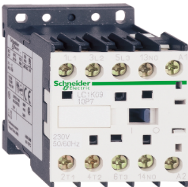
SCHNEIDER ELECTRIC 4KW 9A 1NOV CONTACTOR 48V AC CONTROLLER 3389110374766
