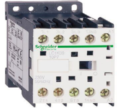
SCHNEIDER ELECTRIC 5.5KW 12A 1NOV CONTACTOR 220V AC CONTROLLER 3389110733129
