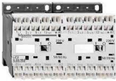
SCHNEIDER ELECTRIC TESYS K INVERTER CONTACTOR 3P(3 NO) AC 3 <= 440 V 9 A 48 V AC COIL 3389118097278
