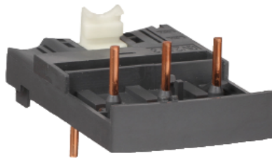
COMBINATION BLOCK FOR COMBINED INSTALLATION OF SCHNEIDER ELECTRIC GV2 WITH LC1-D09?D38 3389110569063
