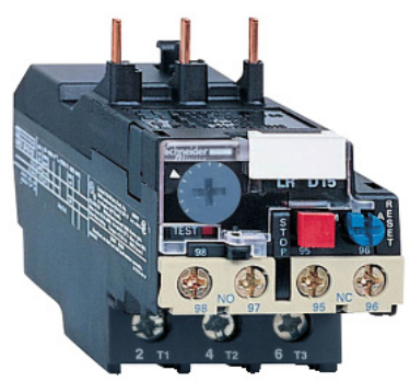
SCHNEIDER ELECTRIC TESIS LRD THERMAL OVERLOAD RELAYS 12...18 A CLASS 20 3389110146745
