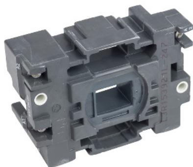
SCHNEIDER ELECTRIC TESYS D CONTACTOR COIL FOR 80 AND 95 A CONTACTOR 24 V AC 50/60 HZ 3389110233353
