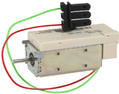
SCHNEIDER ELECTRIC VOLTAGE COIL MN 200..250 V DC/AC 50/60 HZ 3303430473831
