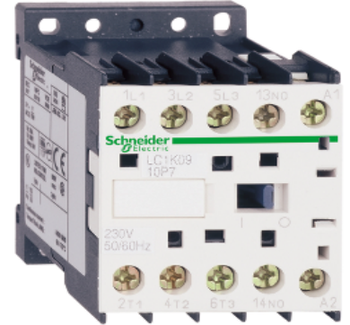
SCHNEIDER ELECTRIC 7,5KW 16A 1NOV CONTACTOR 220V AC CONTROLLER 3389110733136
