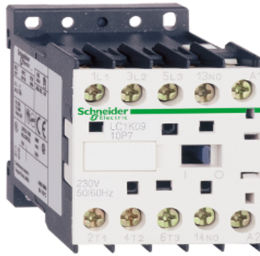
SCHNEIDER ELECTRIC 7,5KW 16A 1NC CONTACTOR 24V AC CONTROLLER 3389110124842
