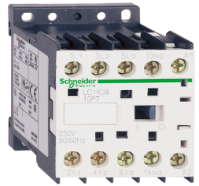
SCHNEIDER ELECTRIC 2.2KW 6A 1NC CONTACTOR 220V AC CONTROLLER 3389110369212
