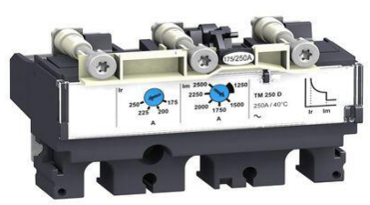
SCHNEIDER ELECTRIC UNITE CUTTING TER-MAG 100A 3F NSX100 3606480017803
