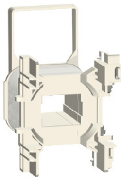
SCHNEIDER ELECTRIC TESYS D CONTACTOR COIL LXD3 48 V AC 50/60 HZ FOR 40...65 A CONTACTOR 3389119410335
