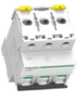
SCHNEIDER ELECTRIC A9F73340 3X40A 6KA B TYPE AUTOMATIC FUSE 3606480079245
