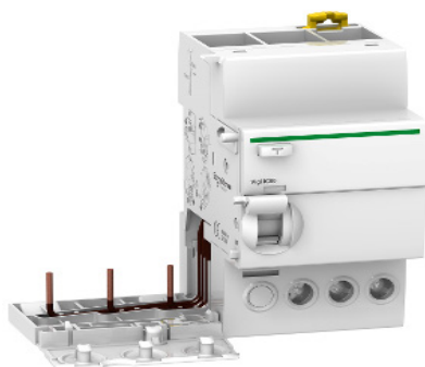
SCHNEIDER ELECTRIC VIGI IC60 EARTH LEAKAGE ADDITIONAL BLOCK 4P 63A 300MA AC TYPE 3606480087455
